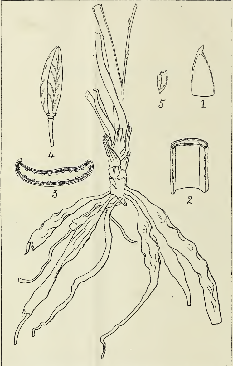
FIG. 1.— Haworthia Blackburniae , Barker, natural size. 1. Tip of leaf \times 4 . 2. Portion of leaf \times 4 . 3. Transverse section of leaf \times 8 . 4. Young fruit \times 4 . 5. Seed \times 8 . (Reynolds 1842 and N.B.G. 1174/36.) Del. W. F. Barker.
